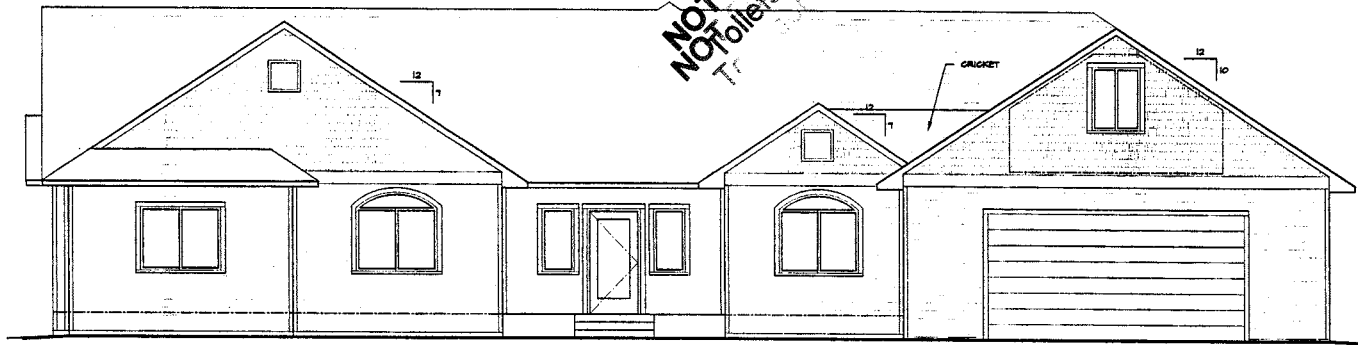
FRONT ELEVATION
