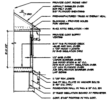
TYPICAL WALL SECTION
