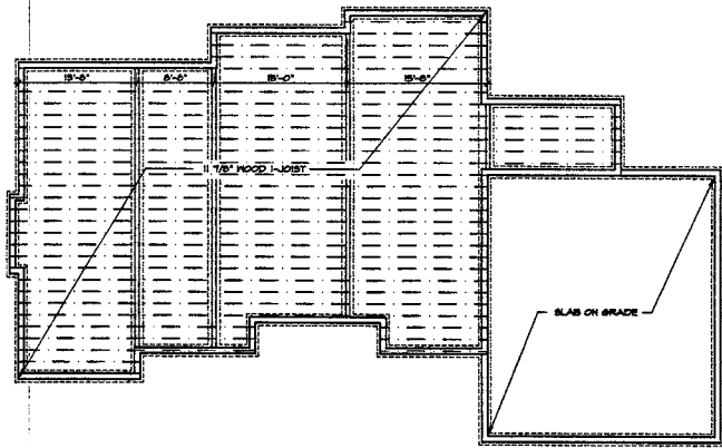
FOUNDATION PLAN
