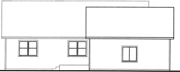
BACK ELEVATION
