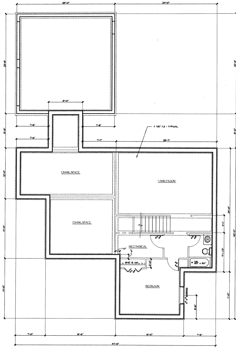
BASEMENT PLAN
