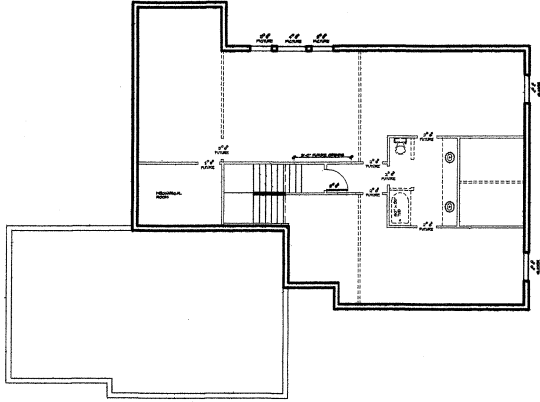
2 BASEMENT FLOOR PLAN 1/8" = 1'-0"
