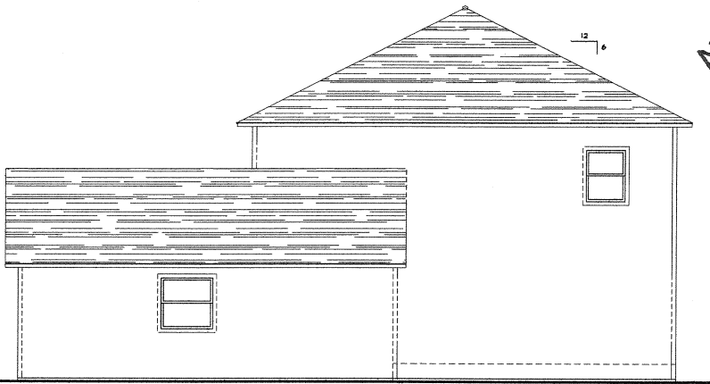
SIDE ELEVATION
