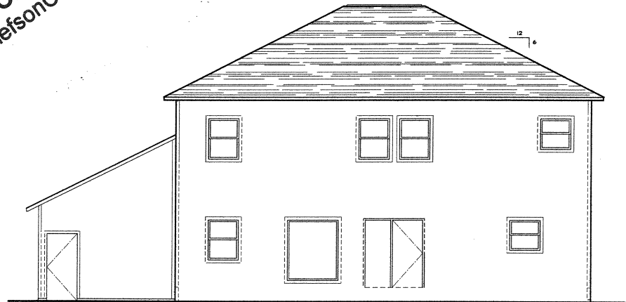
BACK ELEVATION
