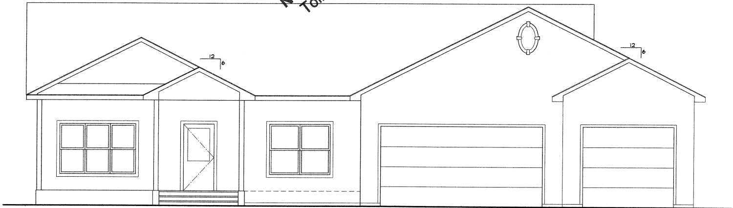
FRONT ELEVATION
