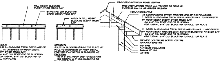
GENERAL WALL - TRUSS CONNECTION
