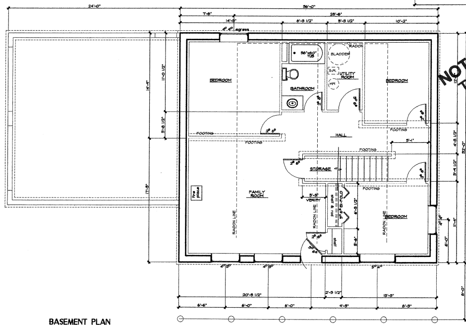
BASEMENT PLAN
