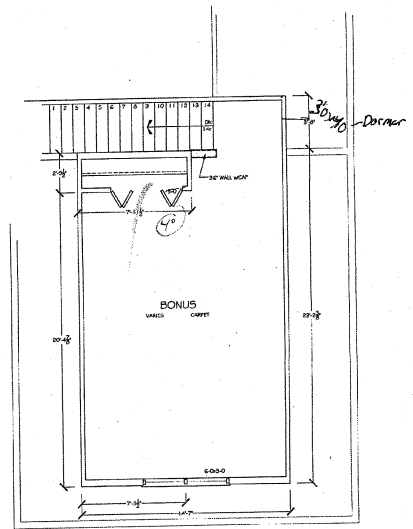
BONUS ROOM PLAN SCALE 1/4" = 1'-0"
