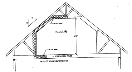
BONUS ROOM SECTION SCALE 1/4" = 1'-0"
