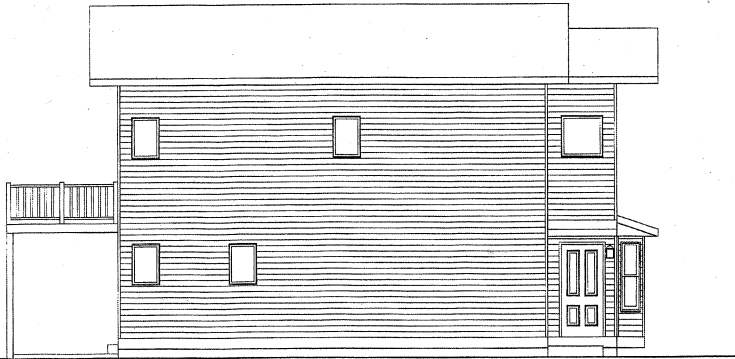
LEFT ELEVATION
