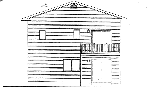
LEFT ELEVATION
